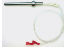
IGNITOR 300W, 120V
