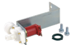
759296CM WATER VALVE 120V, 60Hz single coil. Fits Whirlpool ice machines. Replaces Horton IH3001. Discontinued by OEM.
