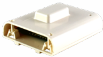
61005988CM ADAPTIVE DEFROST BOARD 120V, 6 pin, discontinued by OEM. Fits older Jen-Air and Maytag refrigerators.
